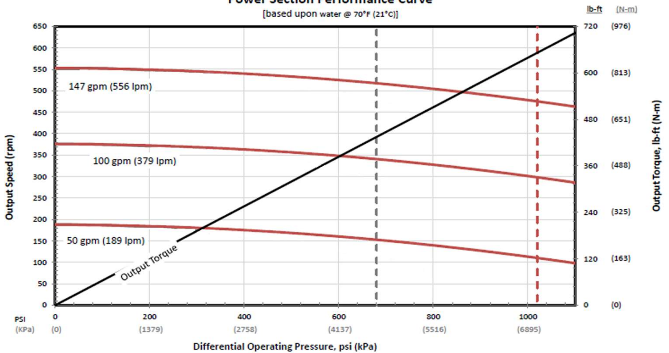
Power Section Performance Curve
